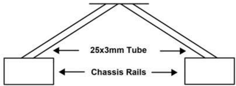
Centre Mount - Group A Rear Wing Rear View
